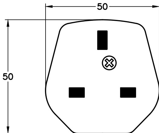
PLUG VIEW
