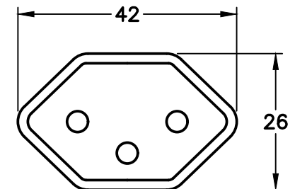
CONNECTOR VIEW
